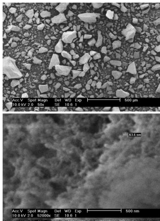
Figure 3. A typical TPAP-doped ormosil (here are shown SEM micrographs of the fully methylated gel B-Me4 ) is made of silica particles ( above ) that upon magnification ( 52,000\times ) reveal a nanostructured spongy morphology ( below ). No changes are observed after reaction in \text{scCO}_2 .
