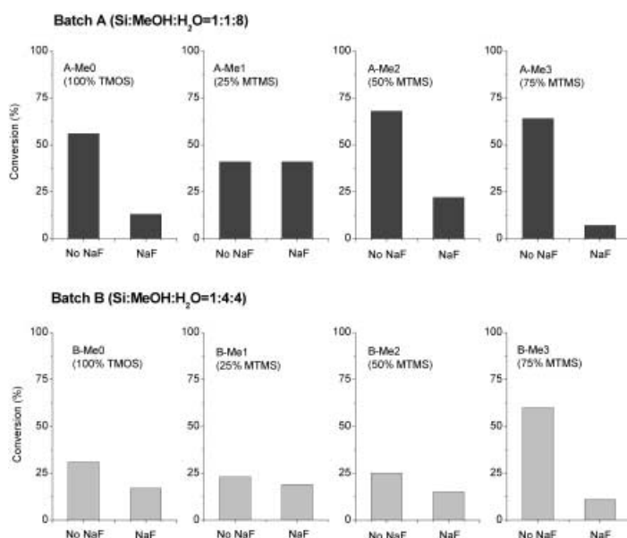
Figure 2. Conversions after 4 h in the aerobic oxidation of benzyl alcohol in \text{scCO}_2 over different gels prepared without (left bars) and with NaF (right bars).
