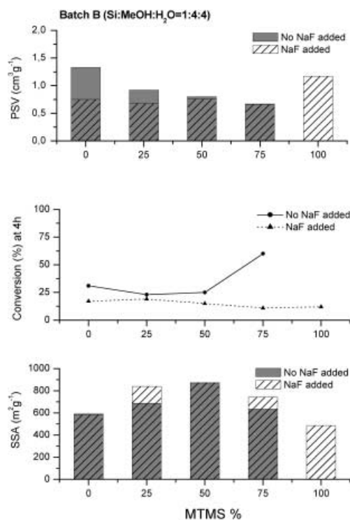
Figure 5. Dependence of the activity of encapsulated TPAP in MTMS/TMOS mixed gels (batch B ) on the gel composition, specific surface area and pore volume.
