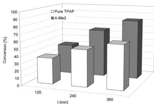
Figure 1. Conversions in the aerobic oxidation of benzyl alcohol in \text{scCO}_2 over TPAP unsupported (white) and entrapped in gel A-Me2 (grey).
