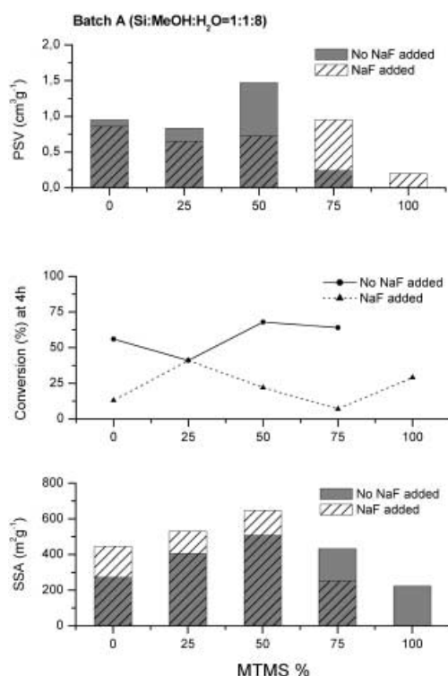
Figure 4. Dependence of the activity of encapsulated TPAP in MTMS/TMOS mixed gels (batch A ) on the gel composition, specific surface area (SSA) and pore specific volume (PSV).
